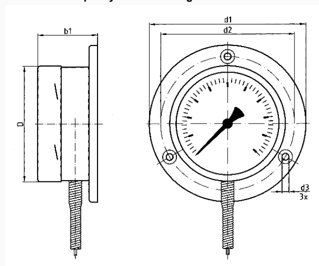
Dimensions (mm)
