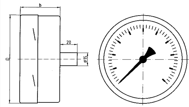
Dimensions (mm)
