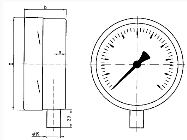
Bottom connection
