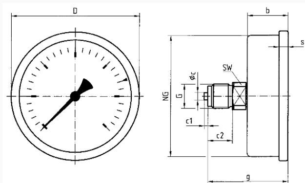
NG 80/100 – centre back connection
