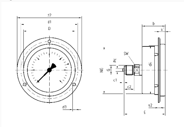
Dimensions (mm)
