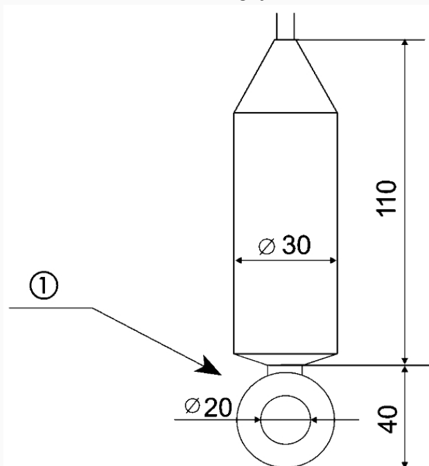
PulsFox® PMG 20 - 62/63 mounting eyelet
