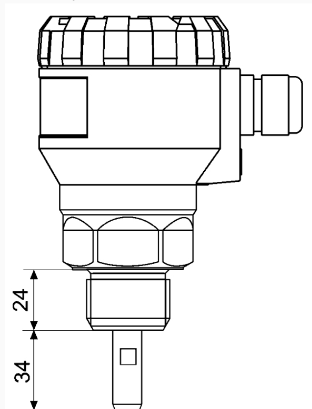
Dimensions (mm)
