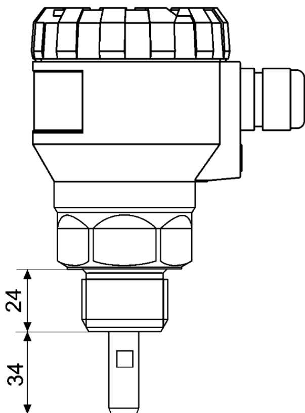
Guided micropulse level indicator PulsFox® PMG 20
