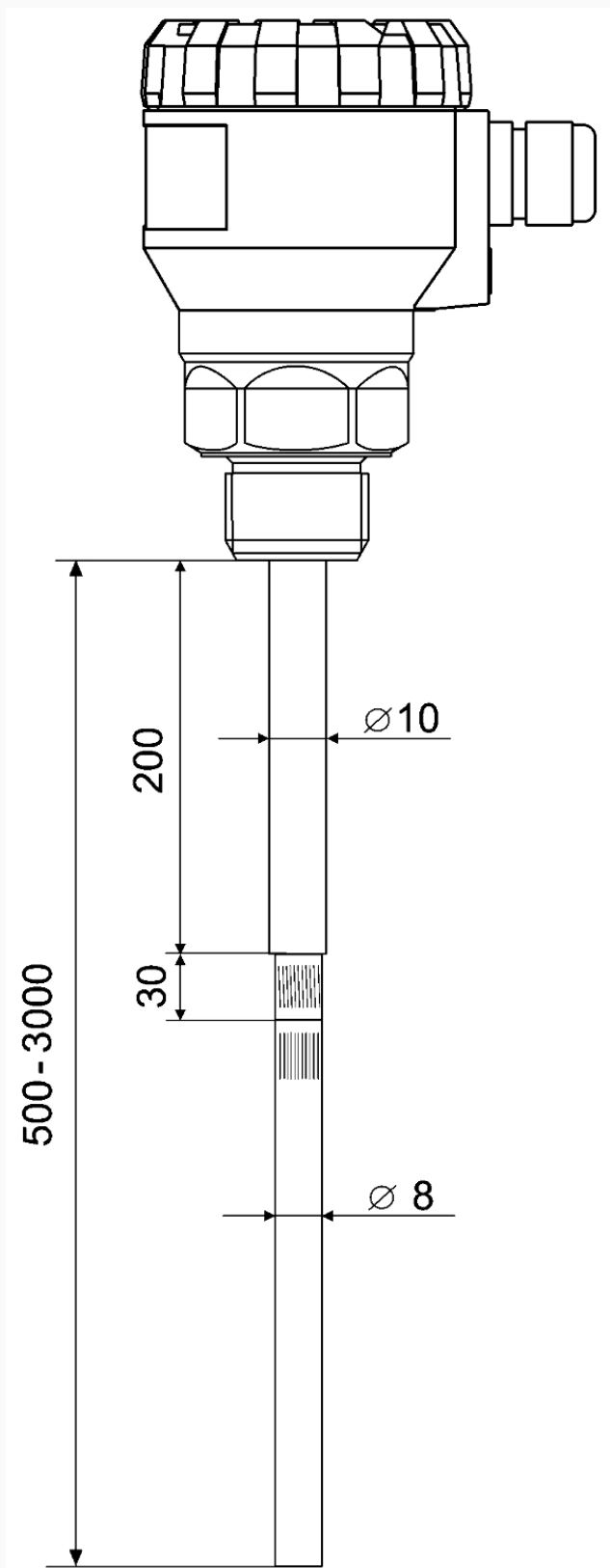
Dimensions (mm)
