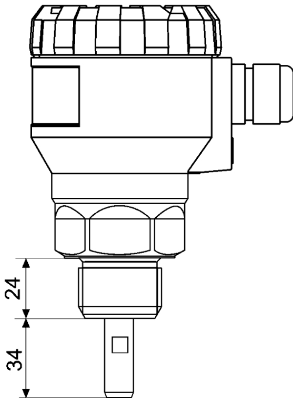
Dimensions (mm)
