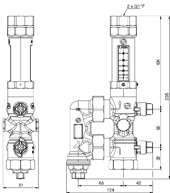
Dimensions (mm)
