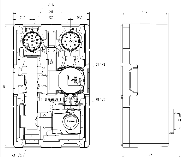
Dimensions (mm)
