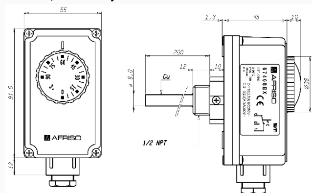
Dimensions (mm)
