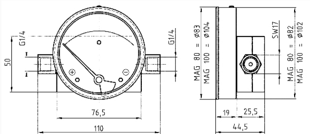
Dimensions (mm)
