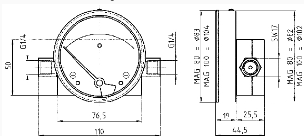
Dimensions (mm)
