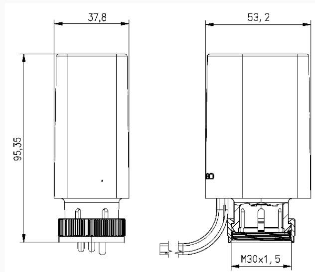
Dimensions (mm)
