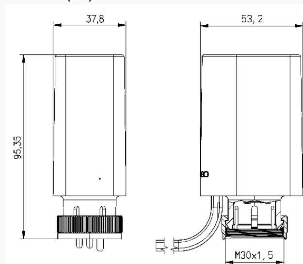
Dimensions (mm)
