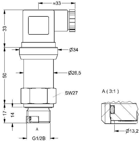
Dimensions (mm)
