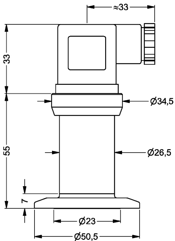
DMU 03 - clamp connection ISO 2852
