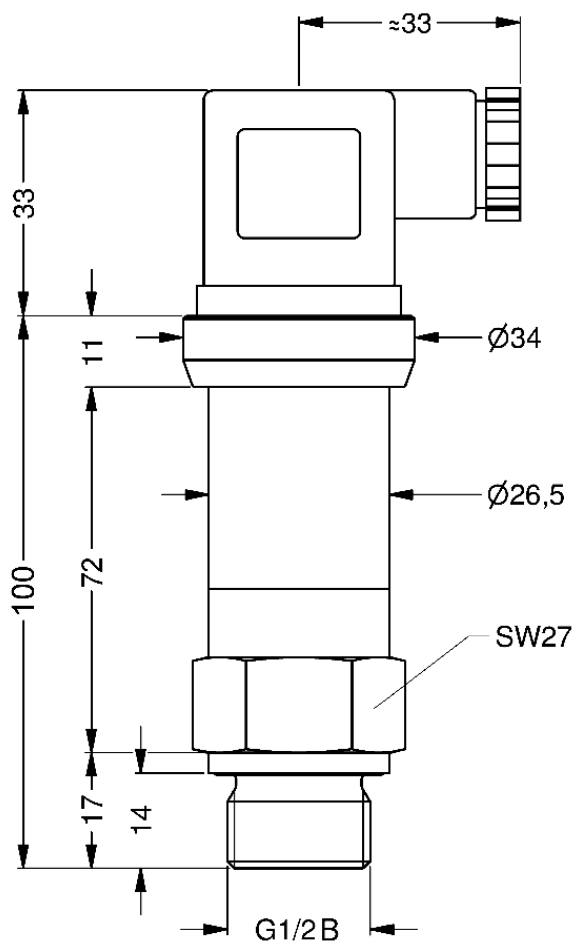
DMU 05 P VM - connection G \frac{1}{2} B DIN 3852 type E with protruding diaphragm
