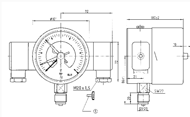
DMU 13 Vario - bottom connection, with electrical contact
