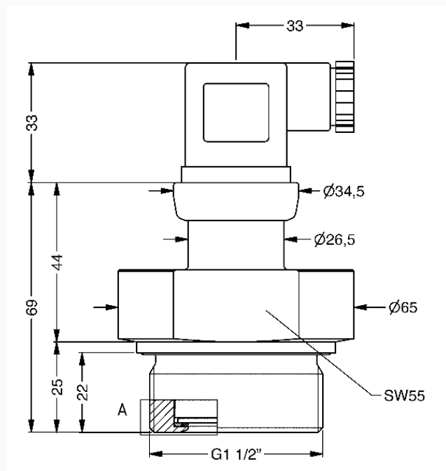
Dimensions (mm)
