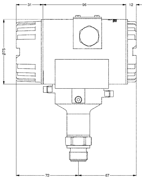
Dimensions (mm)
