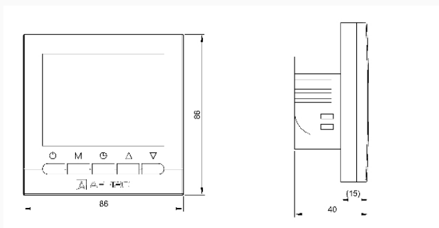
Dimensions (mm)
