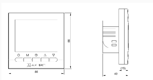
Dimensions (mm)
