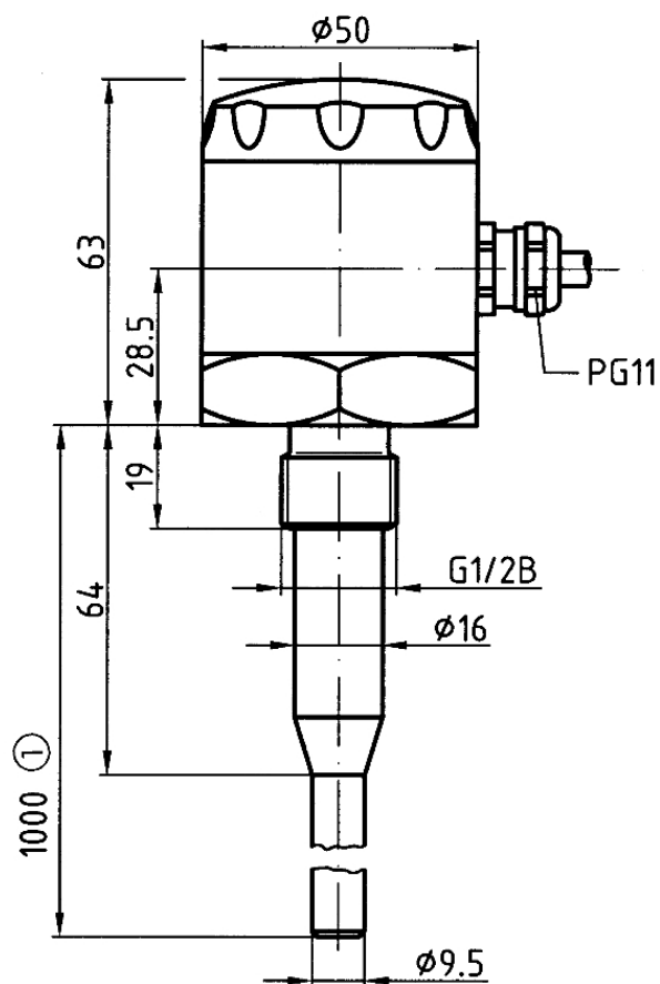
Single-rod probe LST 12
