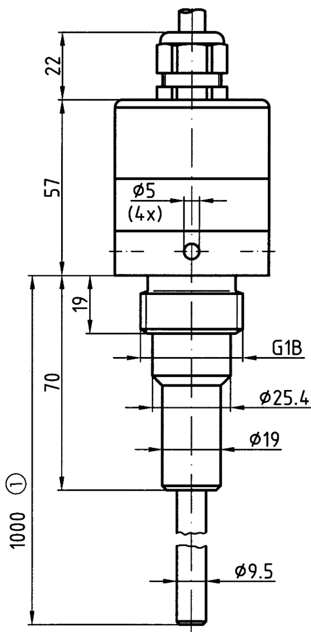
Single-rod probe LST 23
