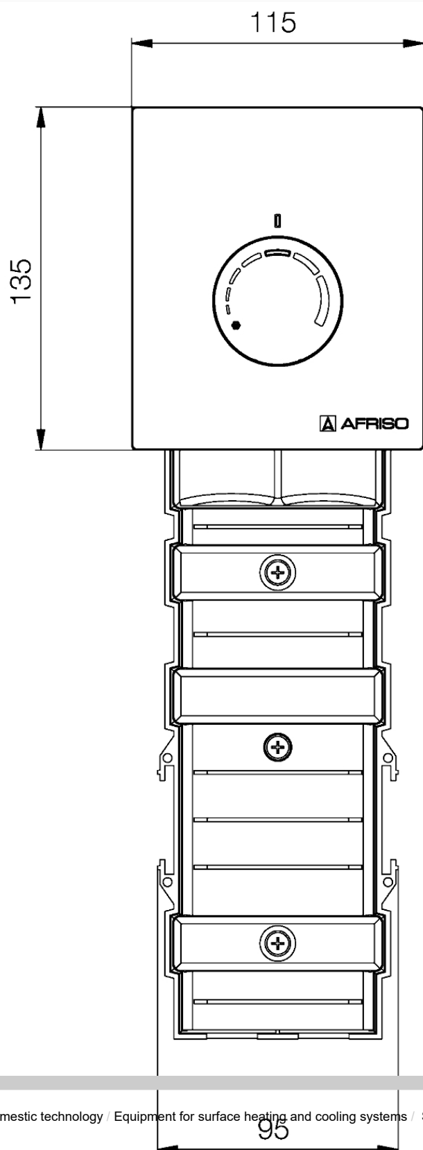
Cover with wall installation box
