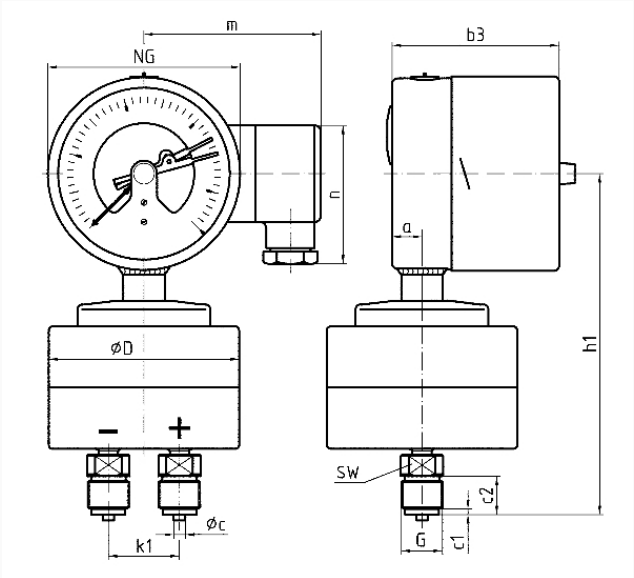
Dimensions (mm)
