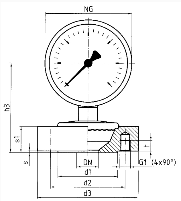
Dimensions (mm)
