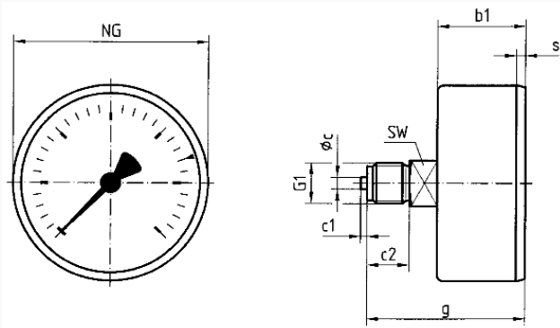
Dimensions (mm)
