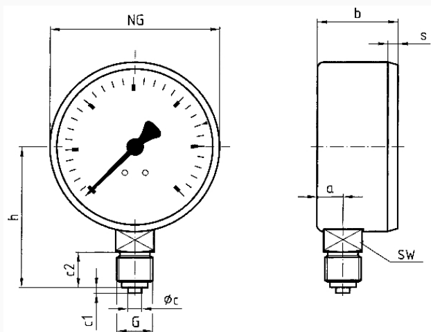
Dimensions (mm)
