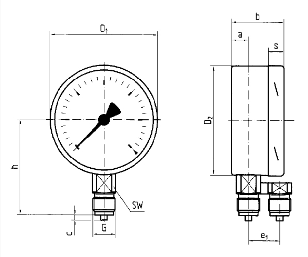
NG 100/160 – bottom connection
