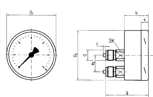
NG 100/160 – centre back connection
