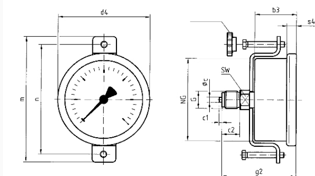
centre back connection, crimped bezel housing with clamp fixing, NG 63
