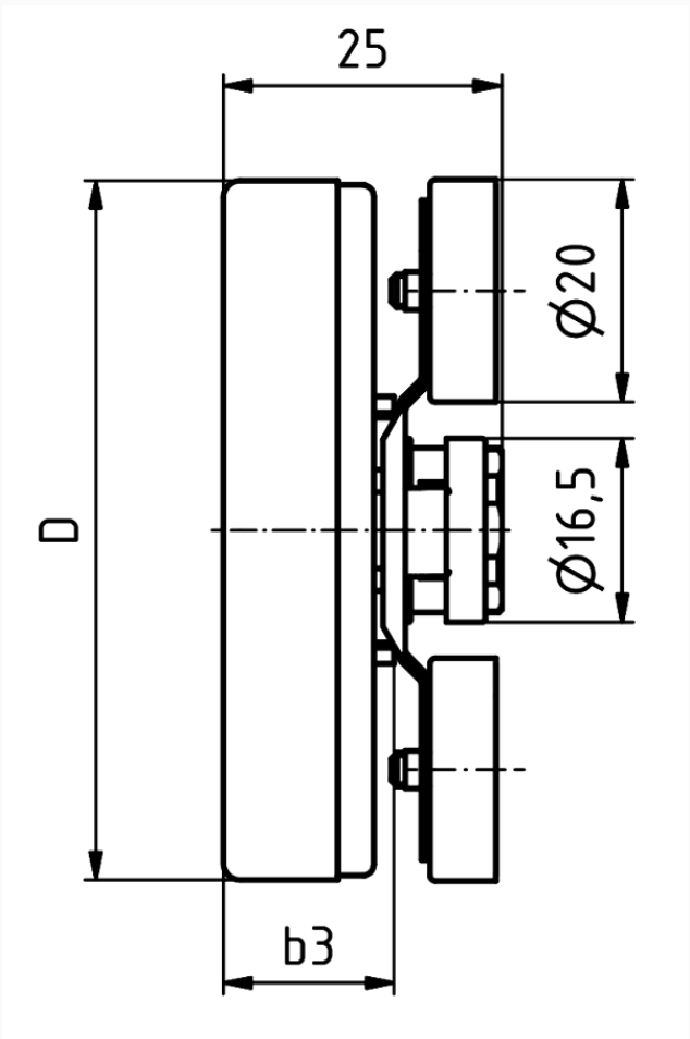
Dimensions (mm)
