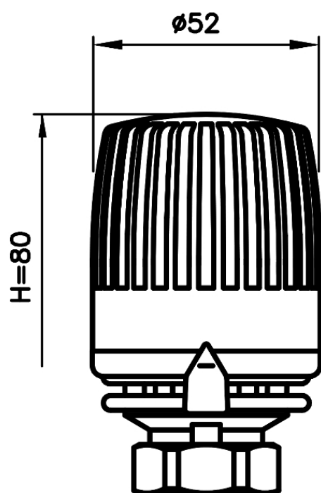
Thermostat control head 323 with fixed probe
