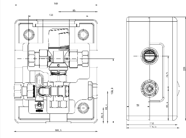
Dimensions (mm)
