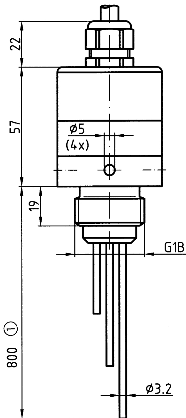
Triple-rod probe LSM 02
