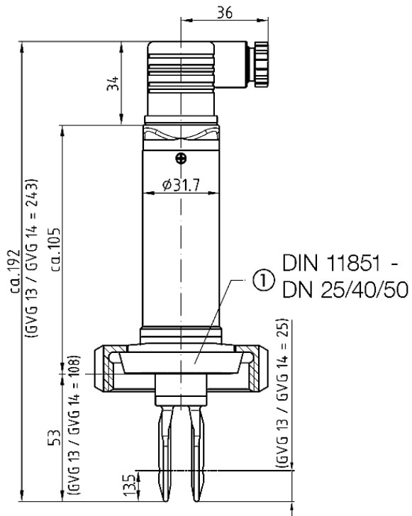
Dimensions (mm) Screwed pipe connection
