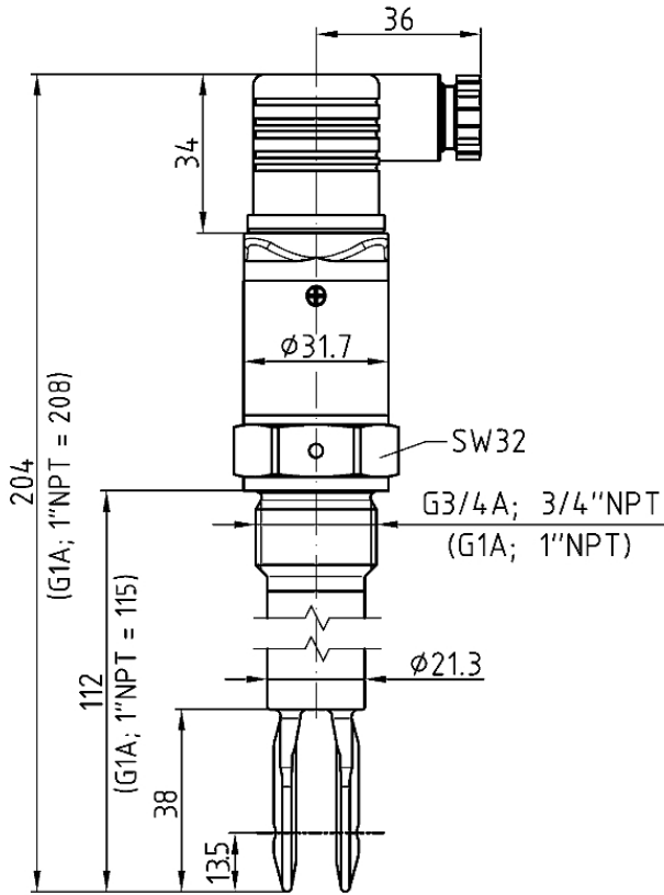
Dimensions (mm)
