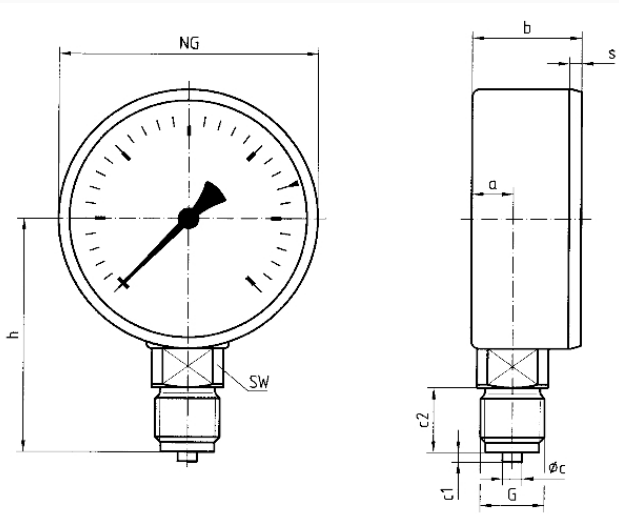
Dimensions (mm)
