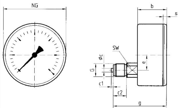
Dimensions (mm)
