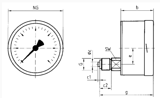
NG 63 – bottom back connection
