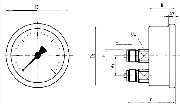
Dimensions (mm)
