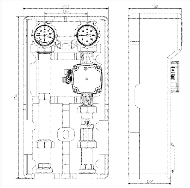
Dimensions (mm)
