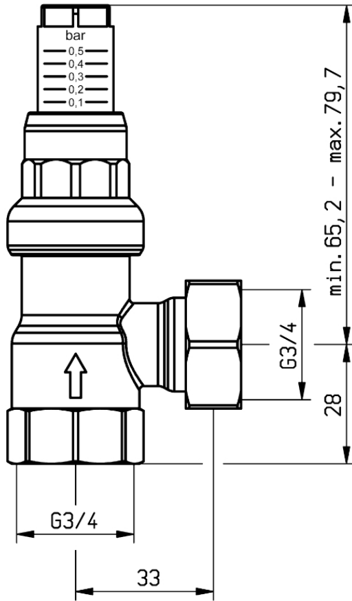
Dimensions (mm)
