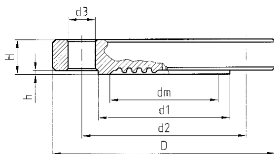
Type MD 80 - flange connection as per EN 1092-1 type B 1
