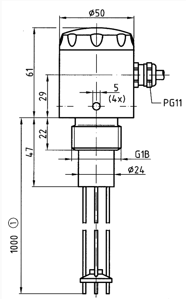
Dimensions (mm) Standard length (can be shortened)
