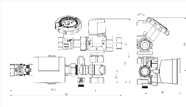
Dimensions (mm)
